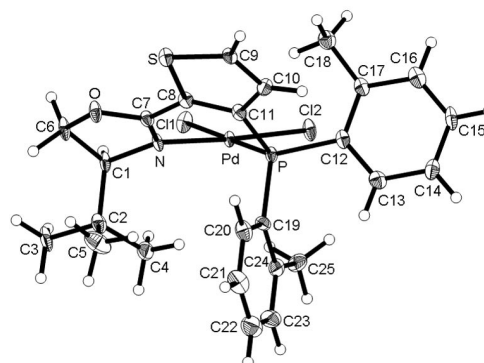
Figure 2. X-ray crystal structure of 16 .
