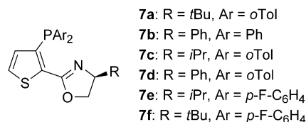
Figure 1. Novel HetPHOX ligands 7c–f .
